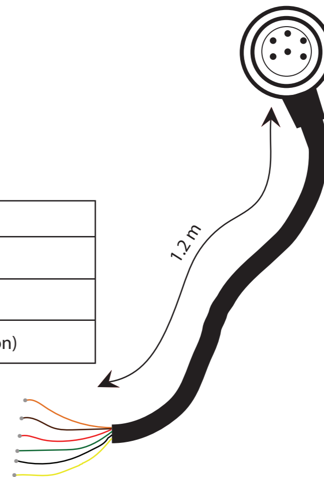
VMPH380190 - Plug Harness for VMEH425200 Series
